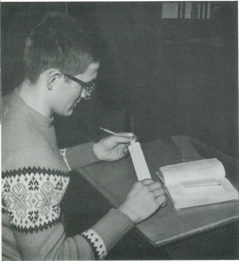
Dale Mosher calculates the x-intercept of a parabola.
