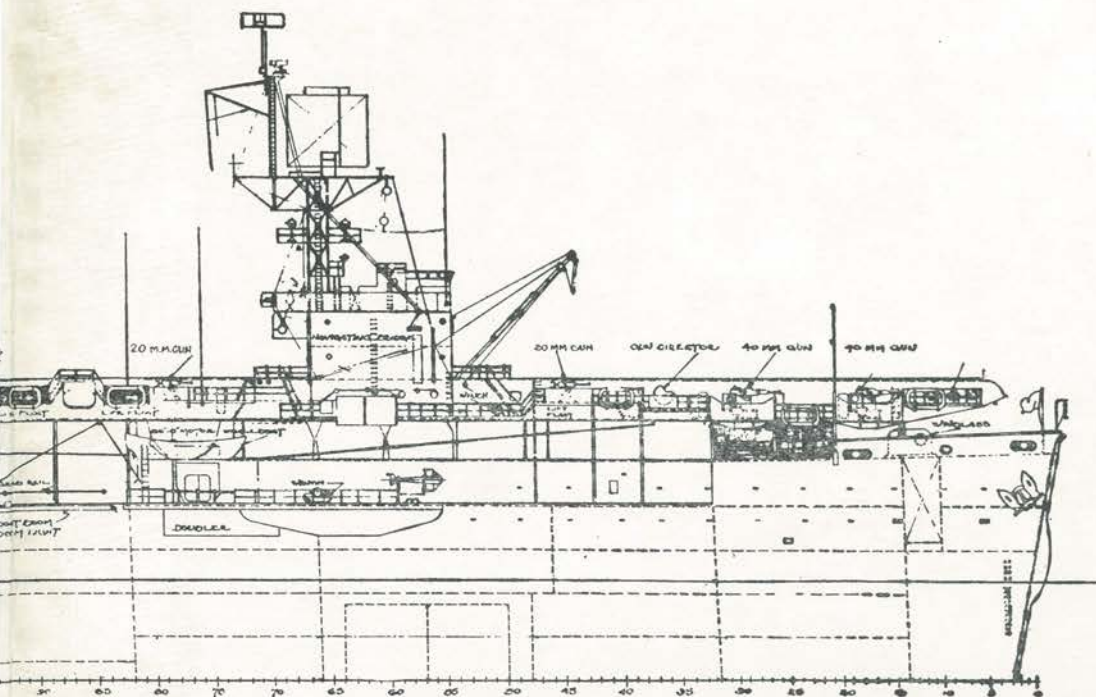
CVE 70 OUTBOARD PROFILE
