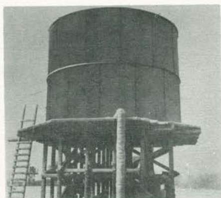
Water Tower (43,000 gals) Morancez
