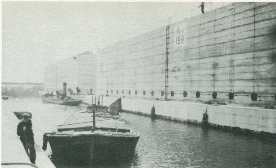
Phoenix being deployed by the British
