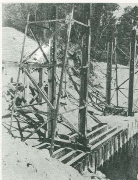
Abutment of adjustable pier, west bank of Irrawaddy River, Ledo Road floating bridge.
