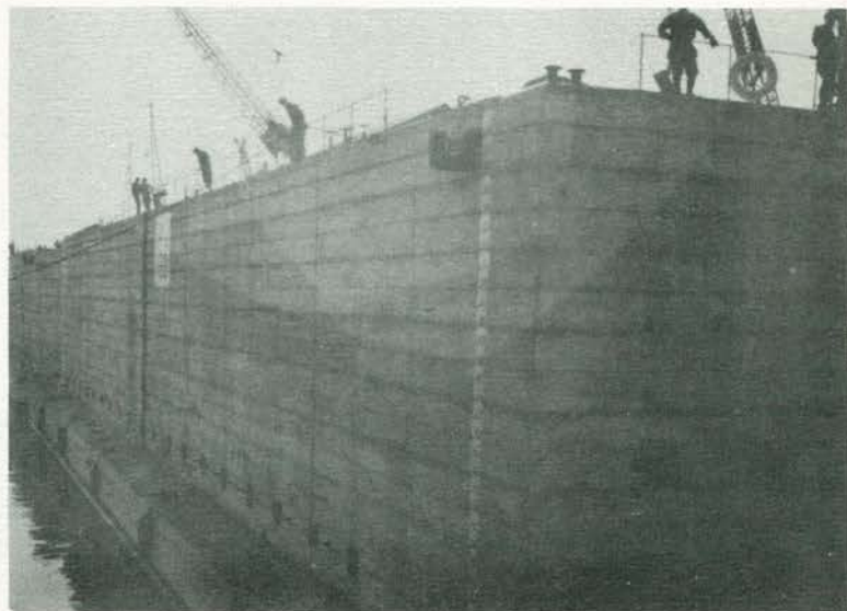
Completed Phoenix
