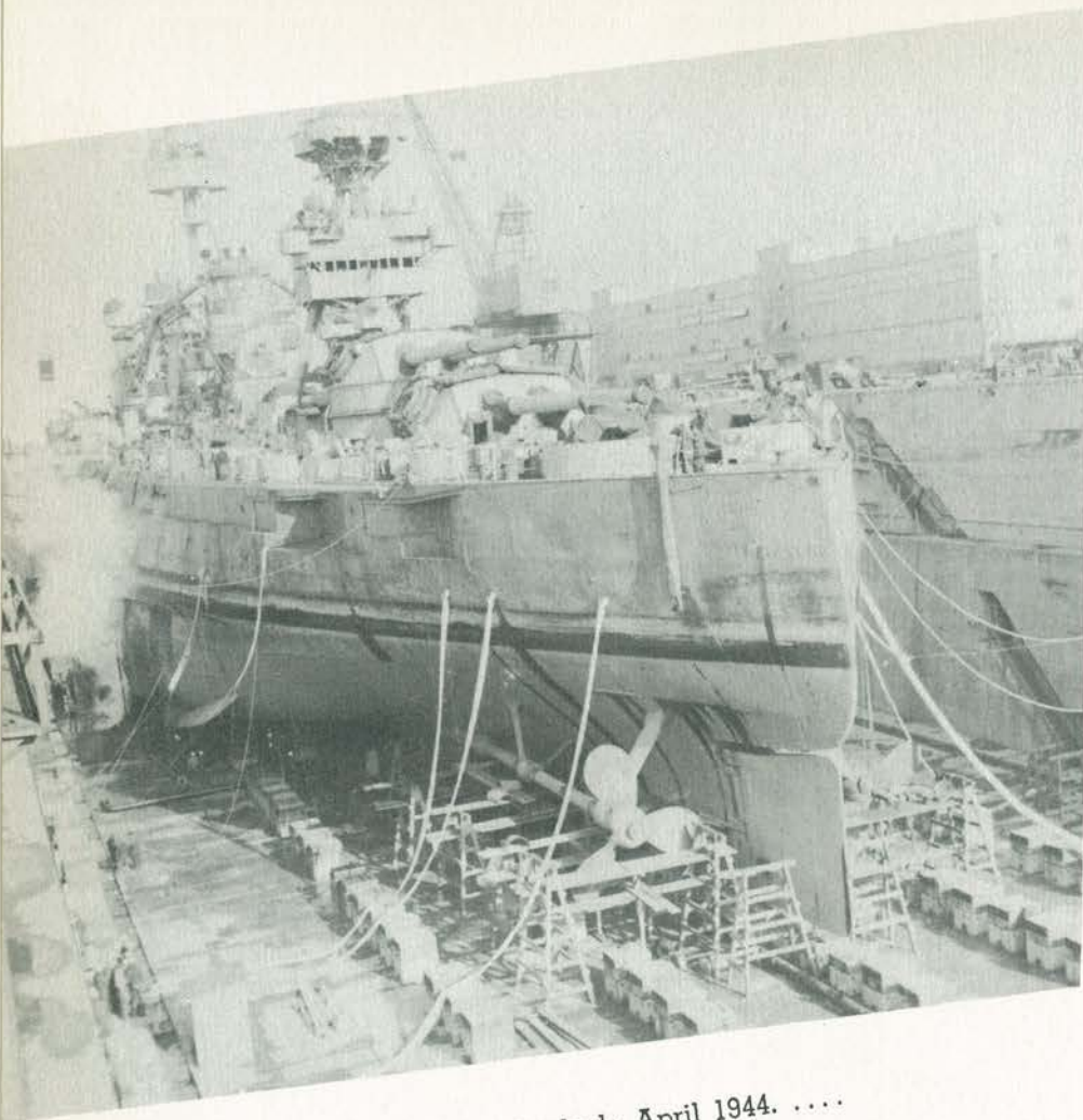
Scraping and wire-brushing the side and underwater bottom meant everybody over the side.
