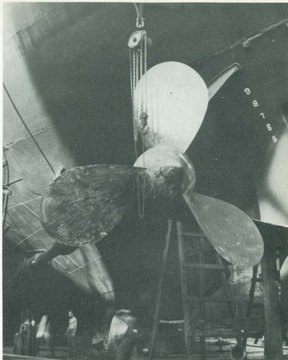
New port screw justifies 1000 mile trip to floating dry dock at Manus.
