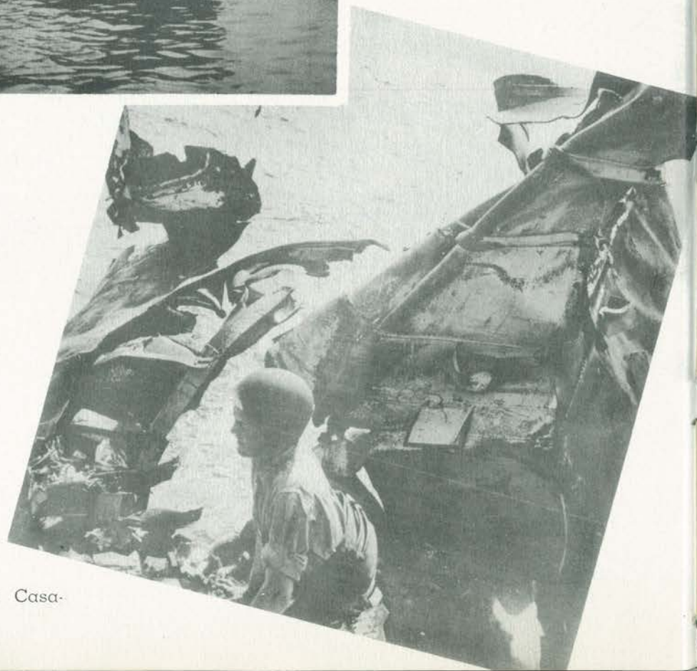
Torpedo Damaged USS Barr Lies In Casablanca Harbor—Her stern a shambles of twisted wreckage, the destroyer escort USS Barr lies in the harbor at Casablanca, French Morocco, where she underwent temporary repairs to enable her to make the voyage back across the Atlantic to Boston. In an Atlantic action May 29, 1944 she was torpedoed by a Nazi U-boat. The escort carrier USS Block Island was sunk in the same battle. The Barr has now been converted into a transport.
