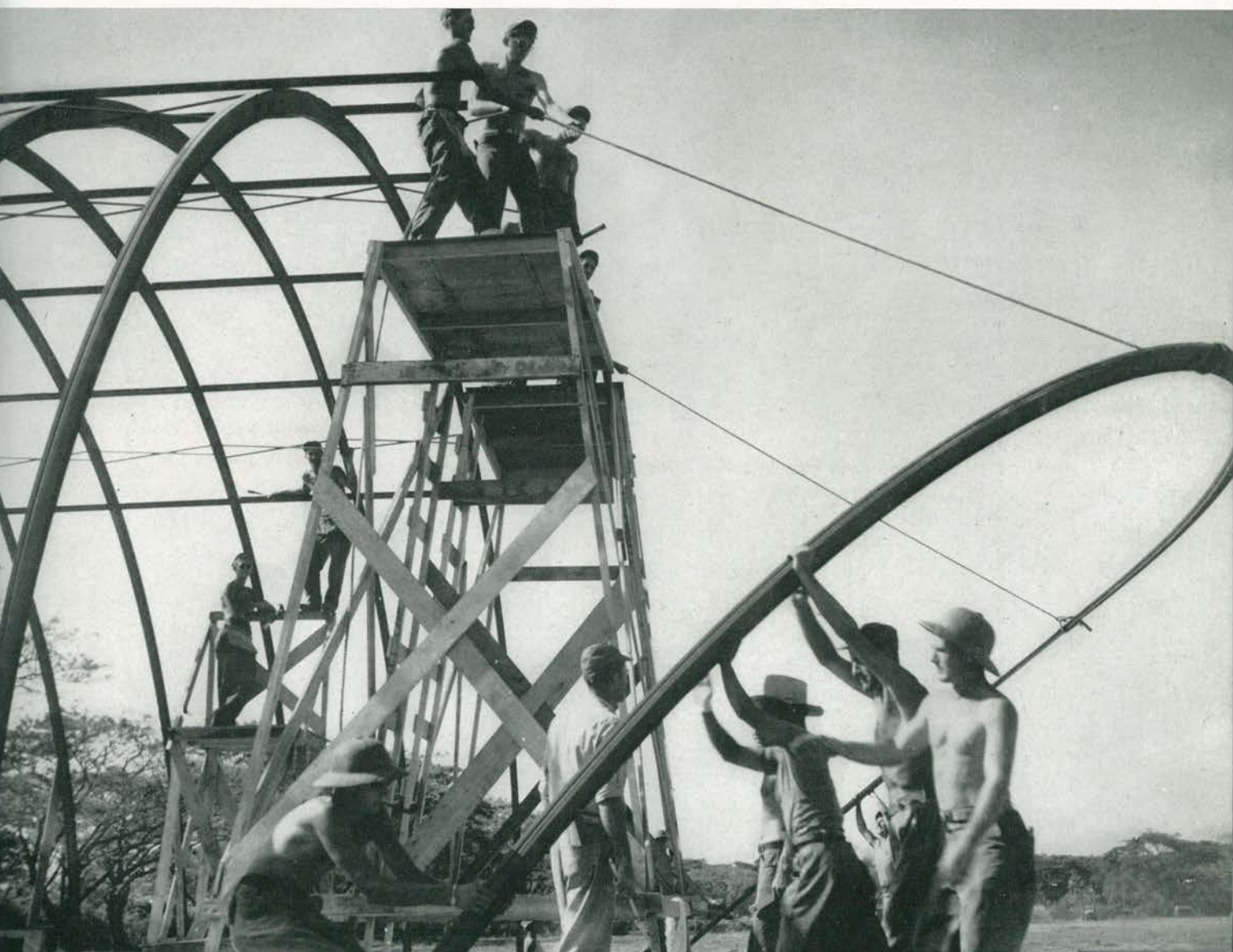
Raising an Arch Rib on a 40' x 100' Quonset Hut.
