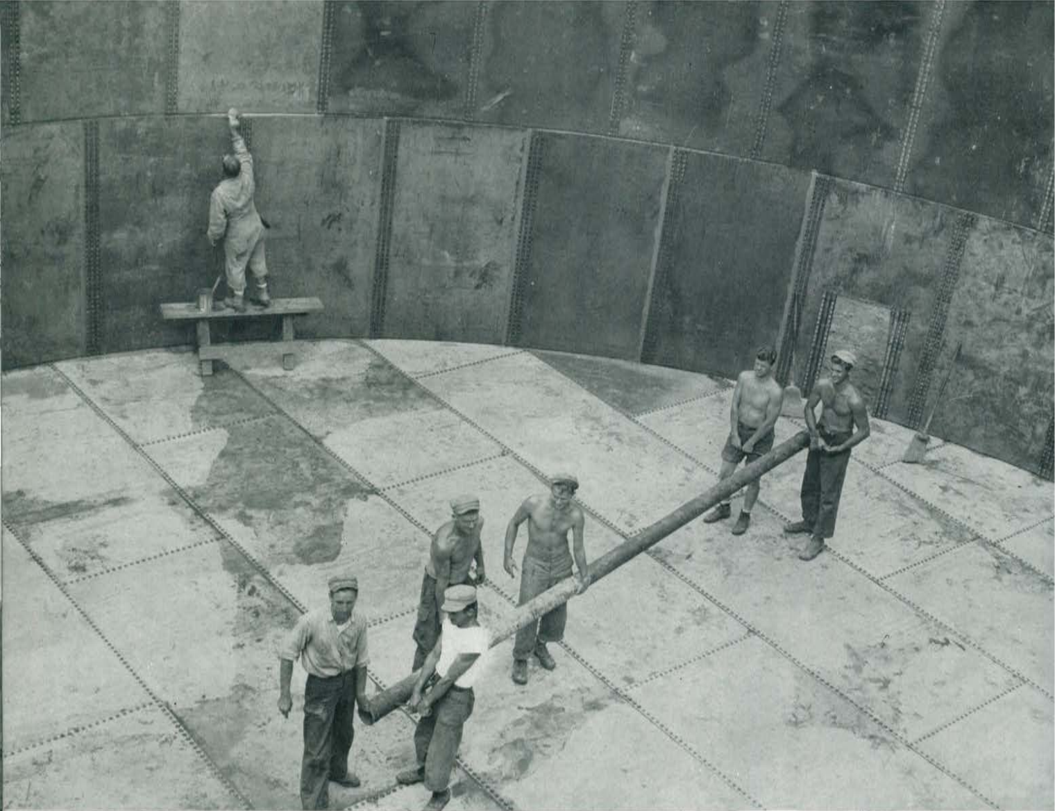
Erecting a steel storage tank.
