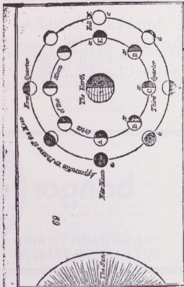
PHASES OF THE MOON.
