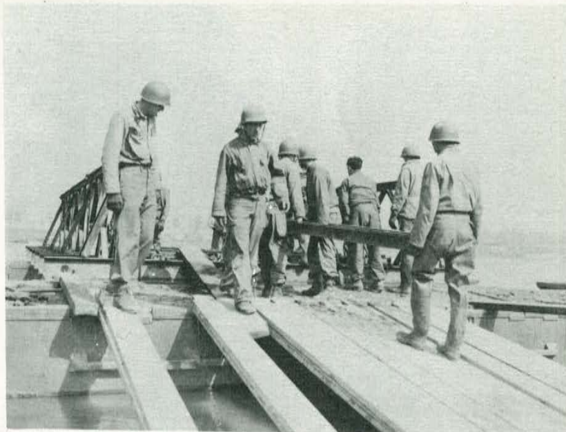
Constructing Floating Bay
