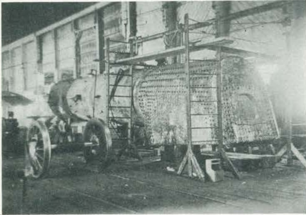
Boiler and fire box section
