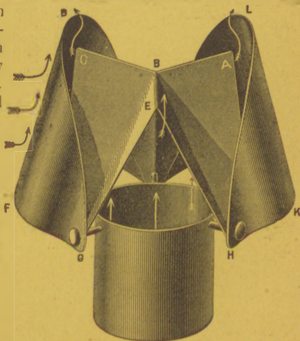
Sectional View of Clover Leaf Ventilator, with one shield removed.
