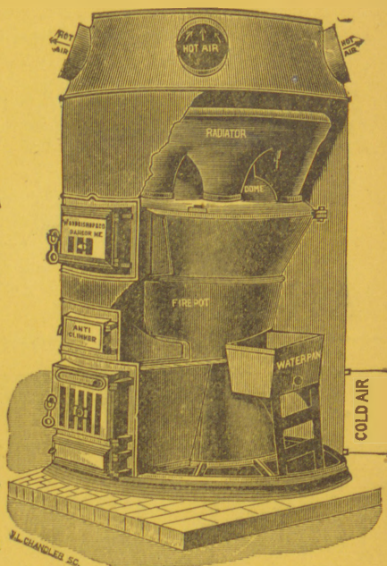
ETNA COAL FURNACE.
