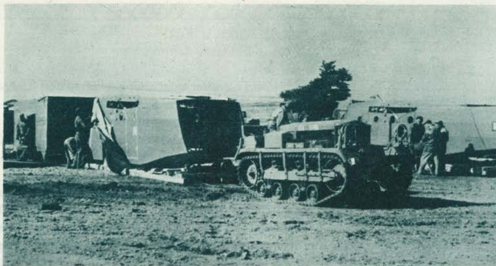
These glider parts arrived in crates on Liberty ships. Cletrac is shown pulling section from a crate.
