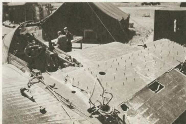
After completing work on Lightning cockpit , men turn their attention to the wings. Picture shows right wing installation.
