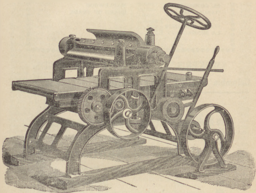
ROTARY BED PLANER.
