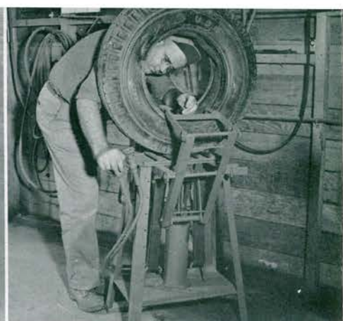
TITMAN TIRE SPREADER
